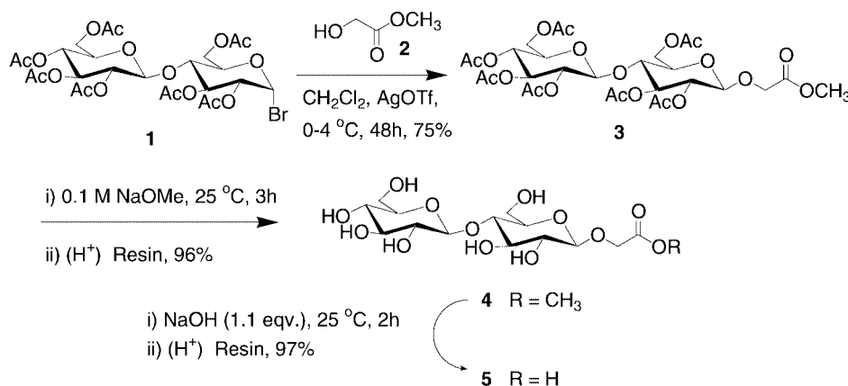
Scheme 1. Synthesis of carboxymethyl \beta -D-cellobioside ( 5 )
