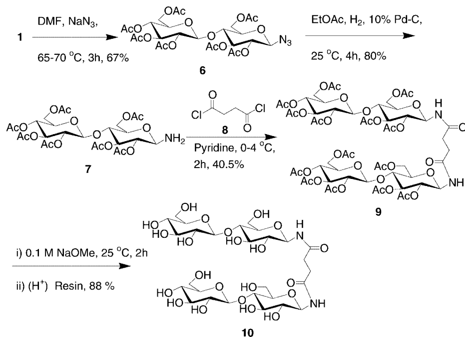
Scheme 2. Synthesis of N,N -bis( \beta -D-cellobiosyl)succinamide ( 10 )
