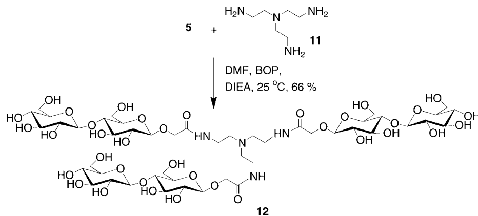
Scheme 3. Synthesis of tris(aminoethyl N -carboxymethyl \beta -D-cellobiosyl)amine ( 12 )
