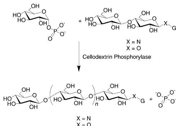
Scheme 9. Enzyme reaction
