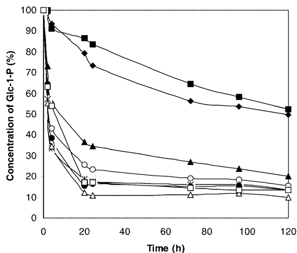
Figure 1. Time course of the CDP reaction with cellobiosylated dimer and trimer and cellobiose-coated PAMAM dendrimers. (◆) 64-mer ( 22 ); (■) 32-mer ( 18 ); (▲) 16-mer ( 18 ); (○) octamer ( 16 ); (*) tetramer ( 14 ); (●) trimer ( 12 ); (△) dimer ( 10 ) and (□) cellobiose.
