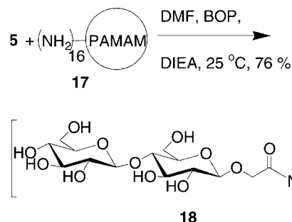
Scheme 6. Synthesis of hexadecameric \beta -D-cellobiosyl PAMAM dendrimer 18
