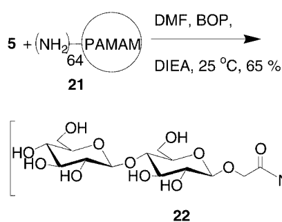
Scheme 8. Synthesis of 64-meric \beta -D-cellobiosyl PAMAM dendrimer 22
